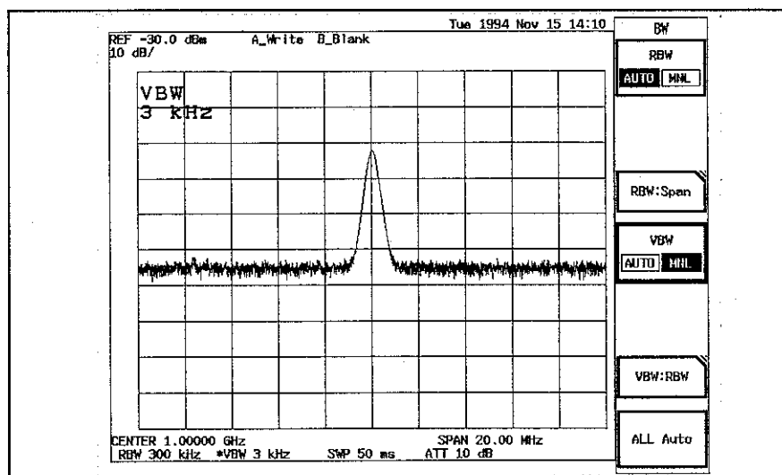
Figure 7-8 VBW = 3 kHz
