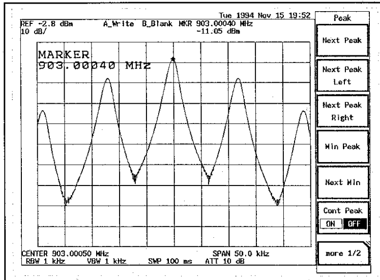
Figure 5-16 Carrier peaks
