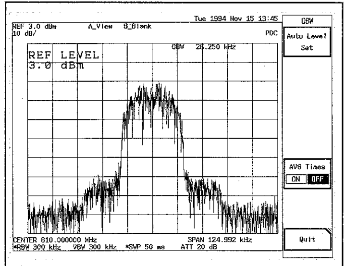
Figure 7-26 OBW measurement screen
