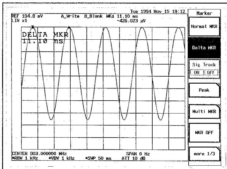
Figure 5-5 Measuring the period of modulated wave
