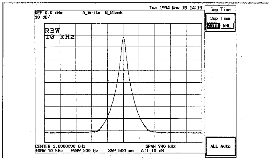
Figure 7-21 SWP = AUTO (500 ms)
