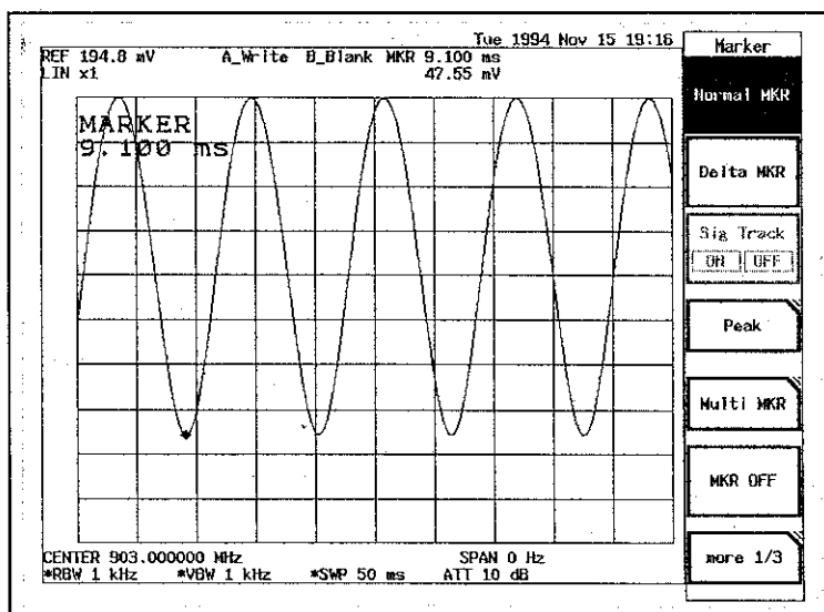
Figure 5-7 Modulation index of AM wave
