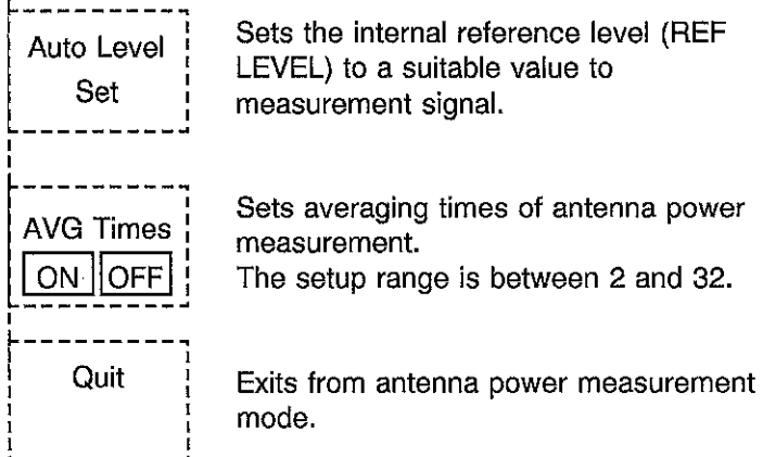
Figure 7-30 Antenna power measurement screen
