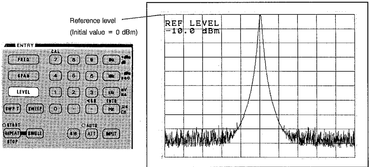
Figure 7-5 Reference Level
