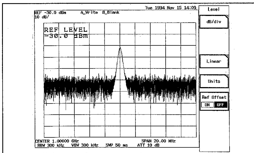
Figure 7-7 VBW = 300 kHz
