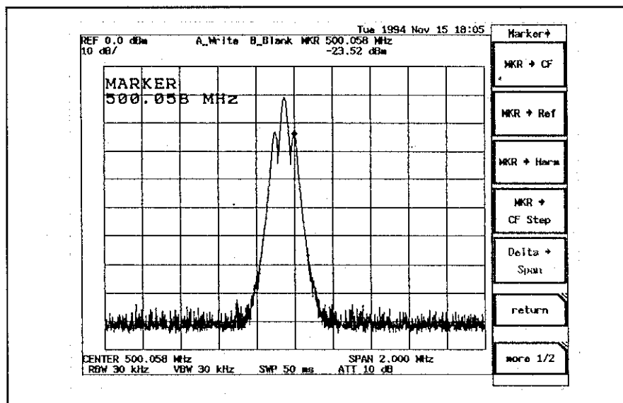
Figure 3-17 MKR⇒CF function
