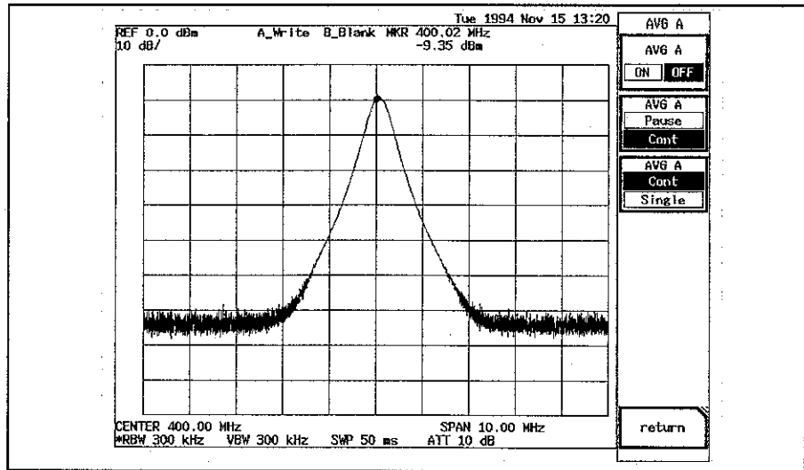
Figure 7-11 No Averaging
