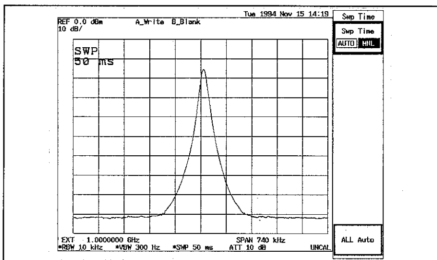
Figure 7-22 SWP = 50 ms
