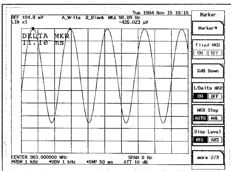
Figure 5-6 Modulation frequency of AM wave
