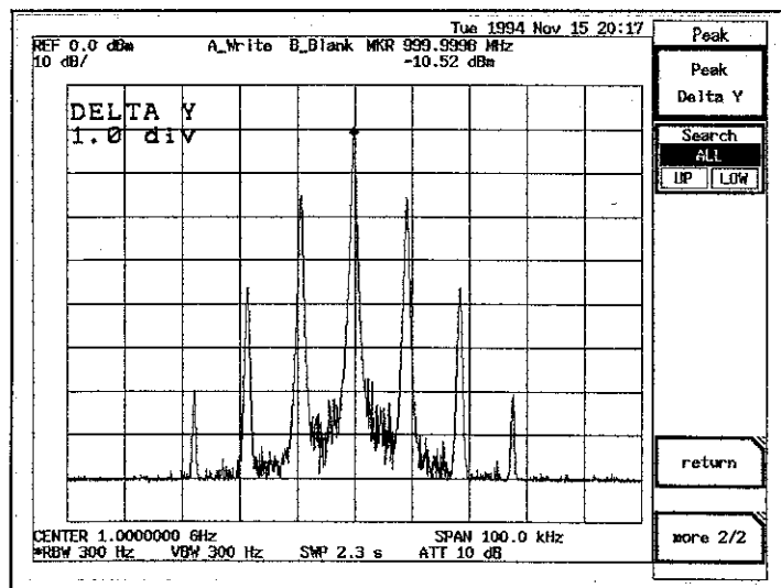
Figure 7-15 Next Peak Search Execution
